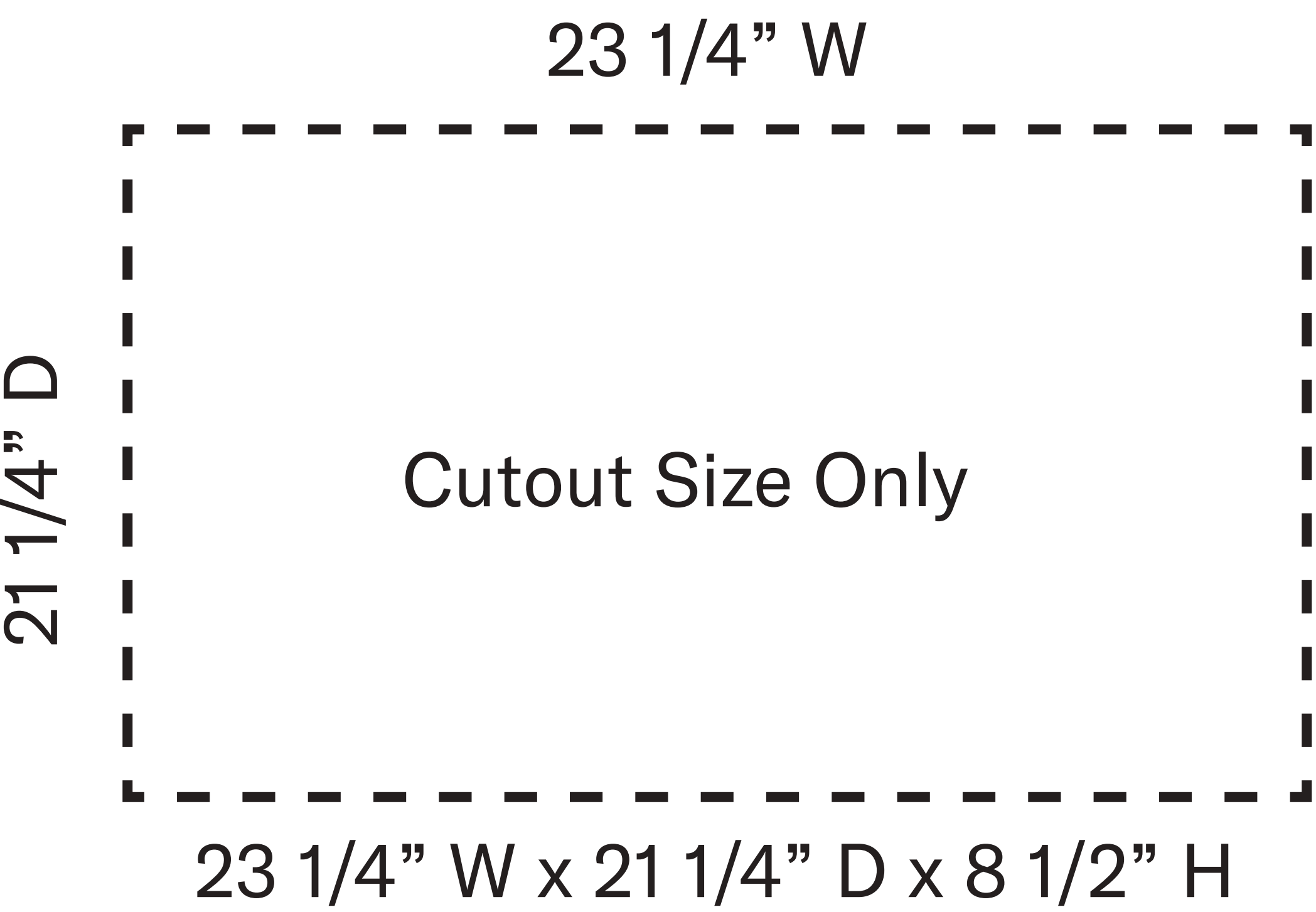
Cutout View
