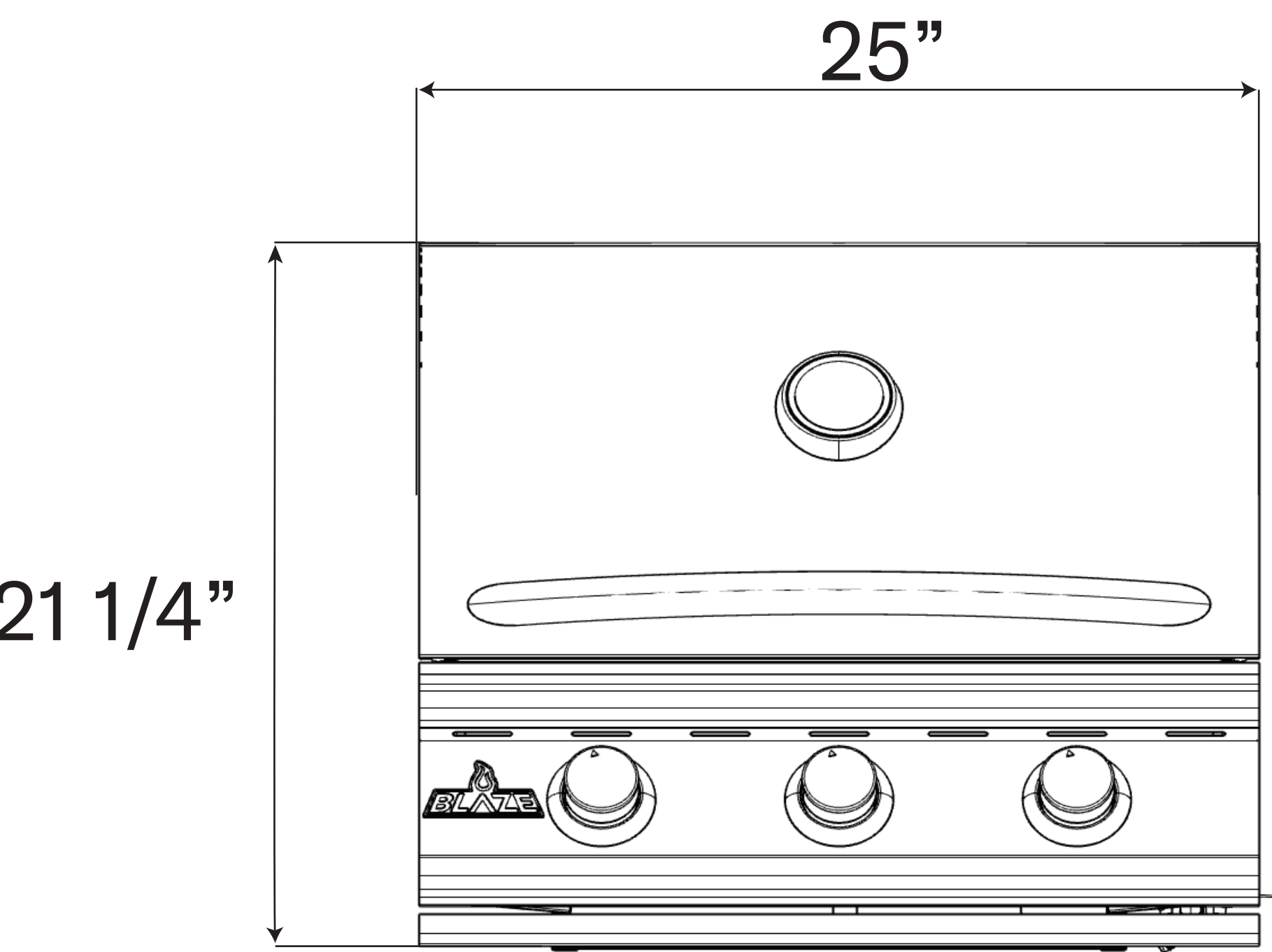
Front View
