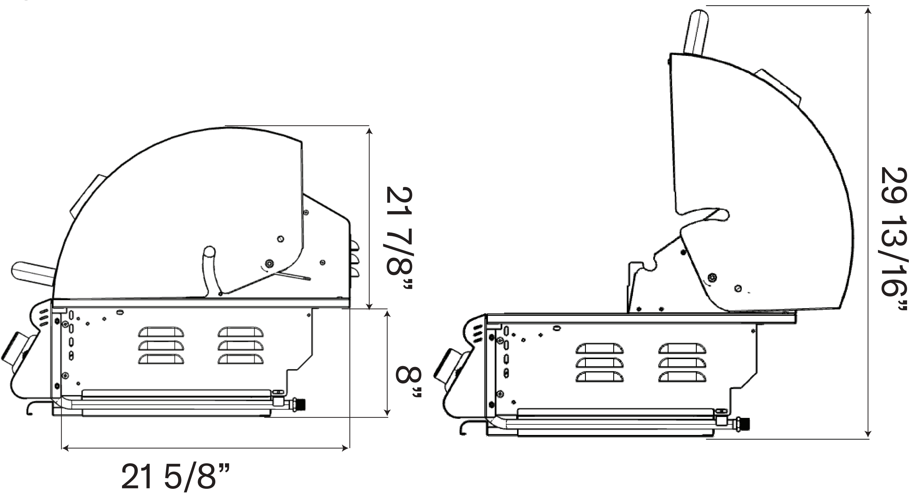
Side View
